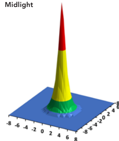
Beam Profile UVG3 2.0 Midlight
