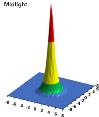
Beam Profile UVG5 2.0 Midlight
