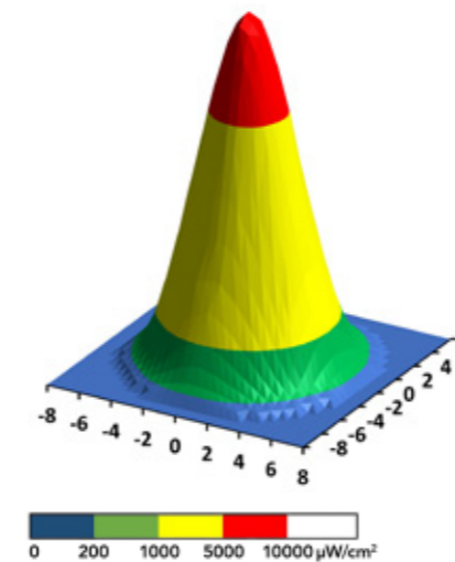
Beam profile MB Poseidon
