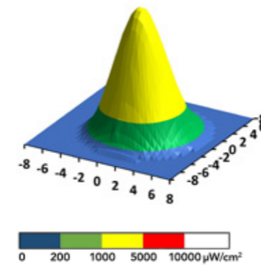
Beam profile MB 3.0 Iris
