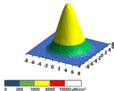
Beam Profile MB PRO Zeus & Hermes
